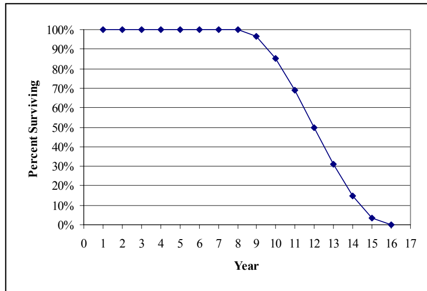
Figure 3.4 Survival Function of Air Conditioners
